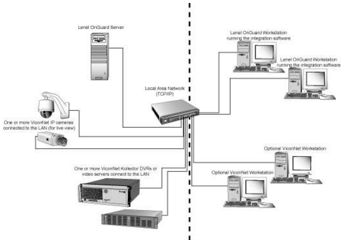
Typical Lenel OnGuard/ViconNet Network Setup
