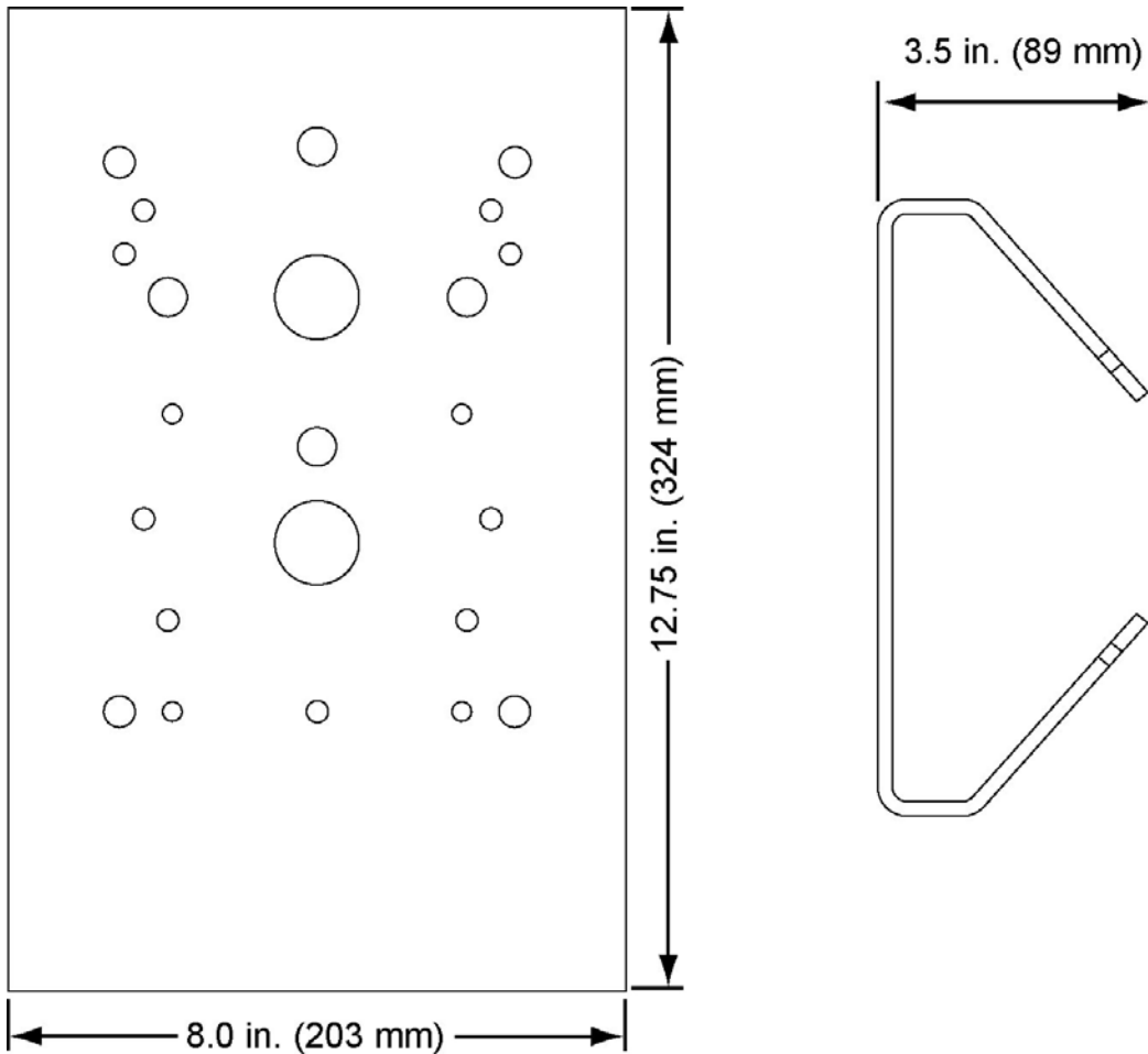
V20B Outline Drawing
